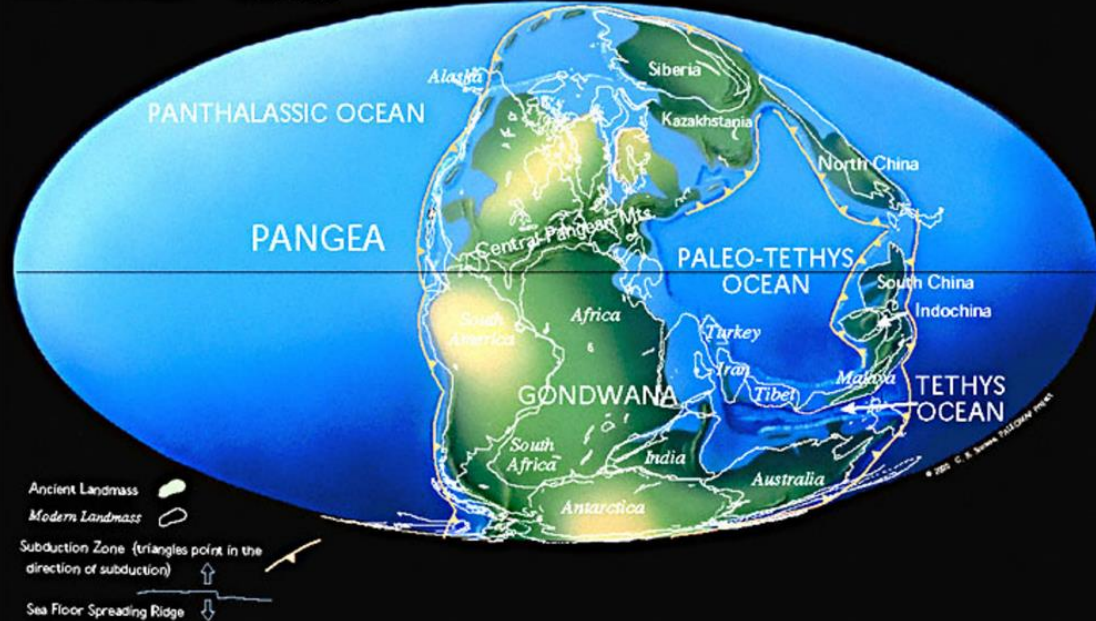
Late Permian 255 Ma
