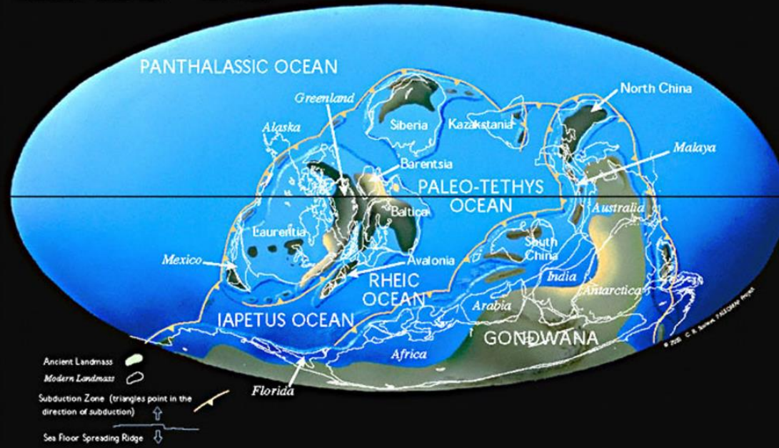
Middle Silurian 425 Ma
