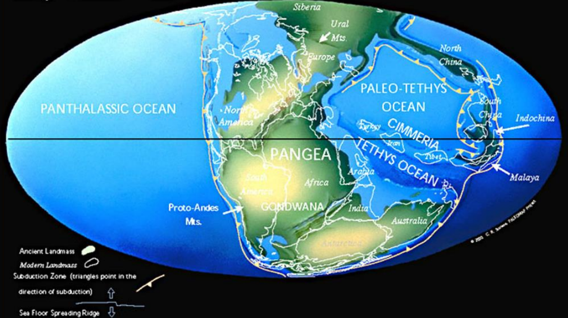
Early Triassic 237 Ma
