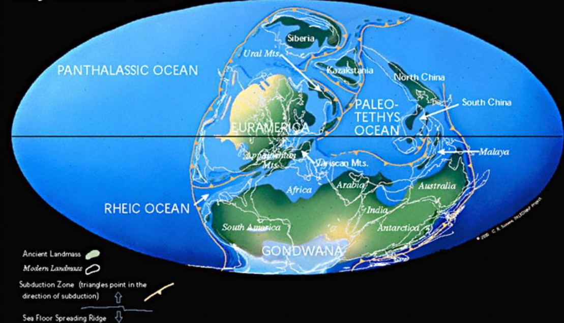
Early Carboniferous 356 Ma
